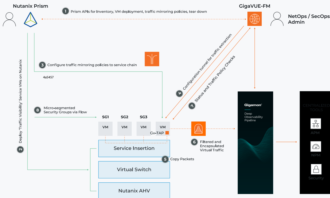
Figure 1. The Gigamon Deep Observability Pipeline is integrated with Nutanix-based private clouds to mirror traffic from all sources, then optimally process and distribute to the appropriate tools.
