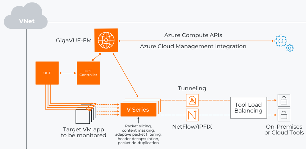
Figure 4. GigaVUE Cloud Suite for Azure is composed of GigaVUE V Series for optimization, transformation, and brokering, as well as GigaVUE-FM for management. For access to workload traffic, GigaVUE Cloud Suite also includes the components UCT and UCT Controller, which are optional, but may be preferred in situations where free workload-level visibility is preferred over paid Azure services.
