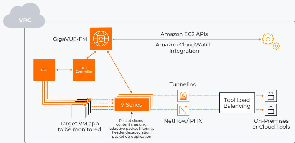
Figure 4. GigaVUE Cloud Suite for AWS is composed of GigaVUE V Series for optimization, transformation, and brokering, as well as GigaVUE-FM for management. For access to workload traffic, GigaVUE Cloud Suite also includes the components UCT and UCT Controller, which are optional, but may be preferred in situations where free workload-level visibility is preferred over paid AWS services.
